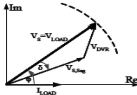
Figure 5. Pre-Sag compensation
